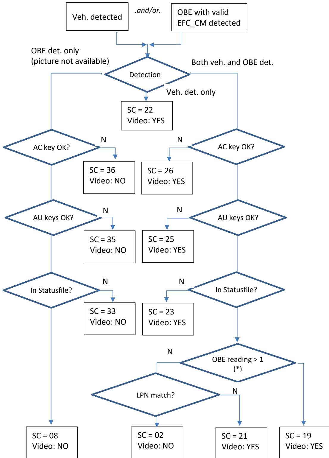
Figure 1: Flow chart of CPE logic
